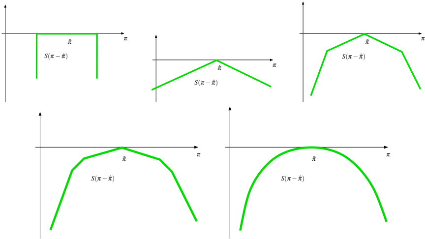
Fig. 13.4 Examples of penalty functions: the boxstep; three piece-wise linear penalty functions; the quadratic penalty of the bundle method.
