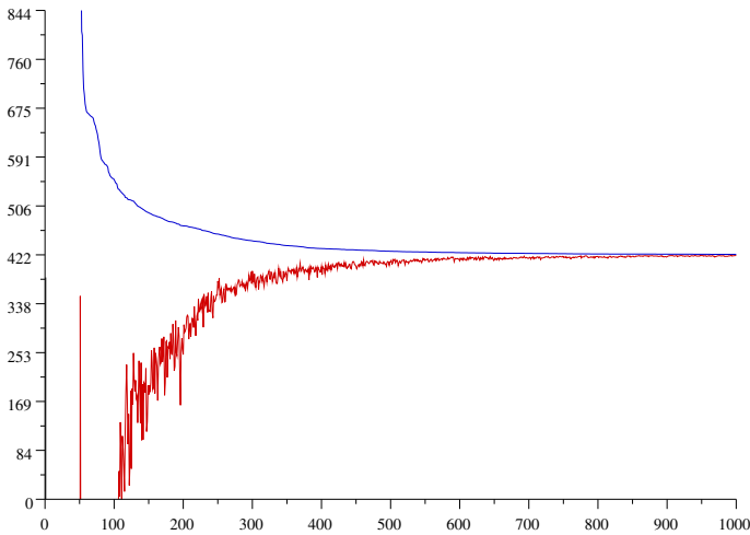
Fig. 13.2 Convergence of the column generation algorithm
