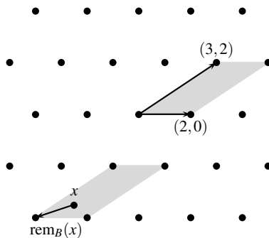
Fig. 14.5 The remainder of a point w.r.t. a basis B .
