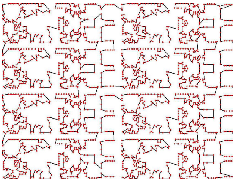
Fig. 12.22 Padberg and Rinaldi's 2,392-city TSP.
