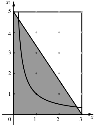
Fig. 15.1 Let K = \{\mathbf{x} \in \mathbb{R}^2 \mid x_1x_2 - 1 \leq 0, 0 \leq x_1 \leq 3, 0 \leq x_2 \leq 5\} . The point (1, 2) is contained in \text{conv}(K_I) . But it violates the constraint x_1x_2 - 1 \leq 0 .
