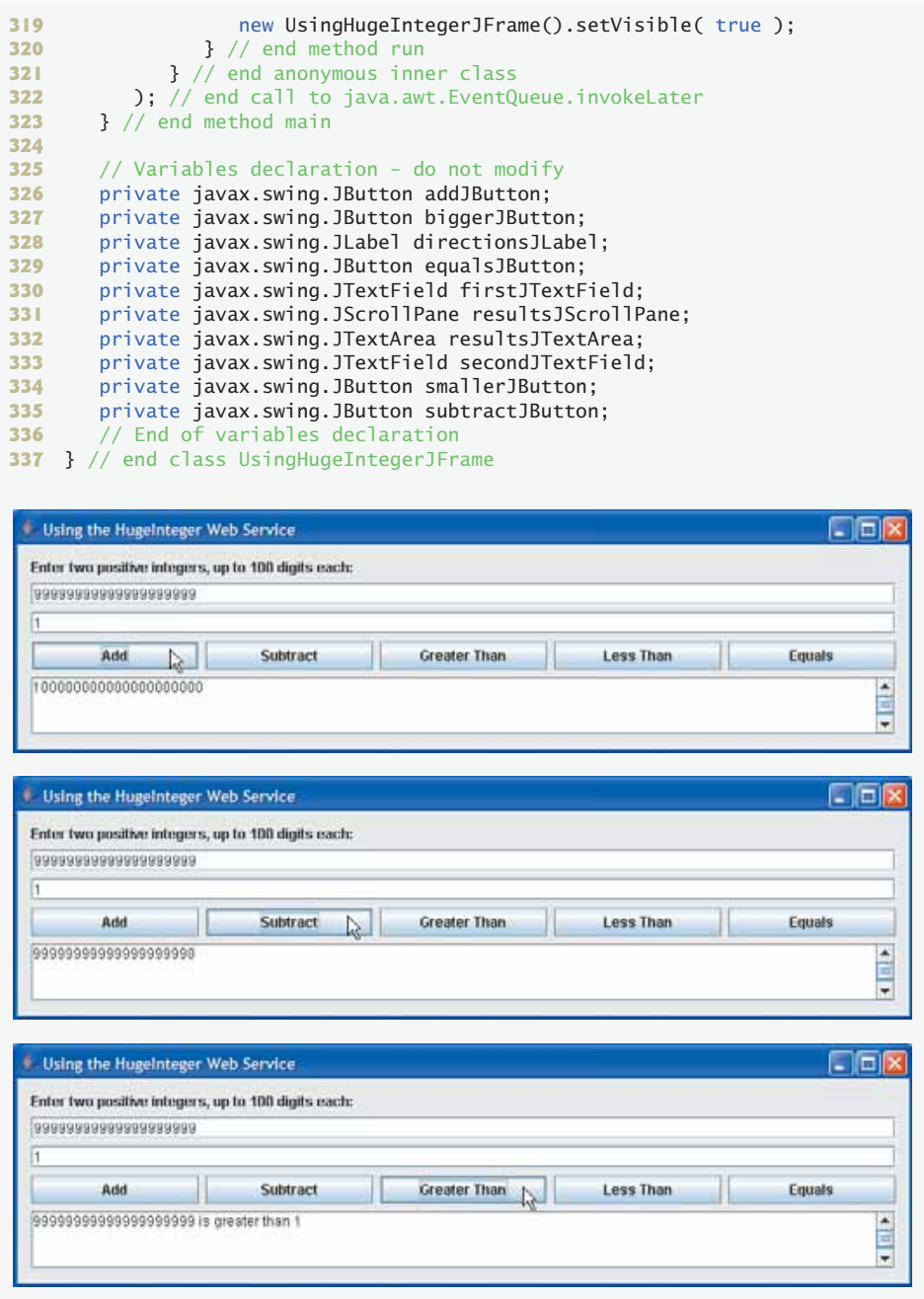
Fig. 28.11 | Client desktop application for the HugeInteger web service. (Part 5 of 6.)
