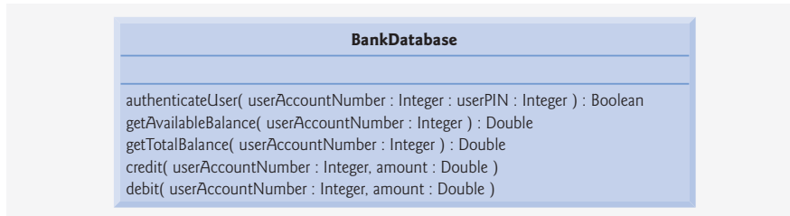
Fig. 6.22 | Class BankDatabase with operation parameters.
